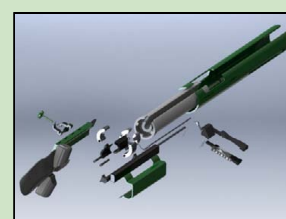
Exploded View
